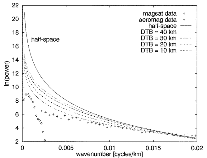
Figure 3. Data of Fig. 1 together with the model power spectra for \beta = 5 .
