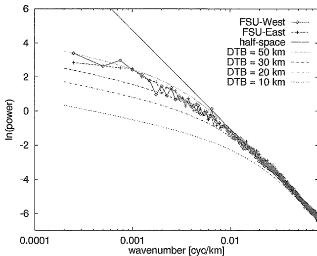
Figure 6. Power spectra of the FSU in log–log scale as in Fig. 5 but with the model power spectra for \beta = 3.5 . The lower the assumed scaling exponent of the crustal susceptibility distribution, the greater the resulting estimate for the DTB.
