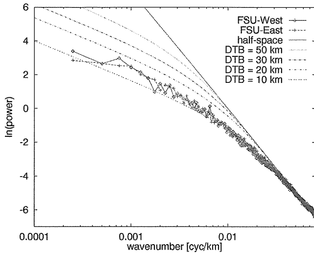
Figure 5. Data of Fig. 4 in log–log scale. At high wavenumbers the magnetic field is self-similar and its log–log power spectrum is a straight line. At wavelengths above 50 km (corresponding to wavenumbers below 0.02 \text{ cycles km}^{-1} ) the power is decreased due to the limited depth extent of the crustal magnetization. The model indicates a DTB of about 15 km under the assumption of \beta = 4 .
